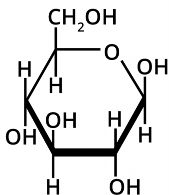
Glucose
